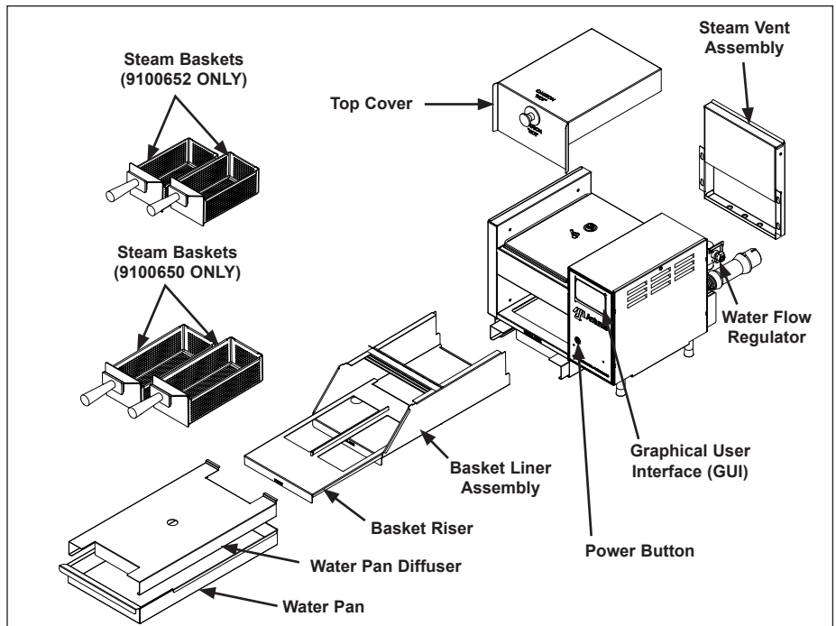
Figure 1. Components
