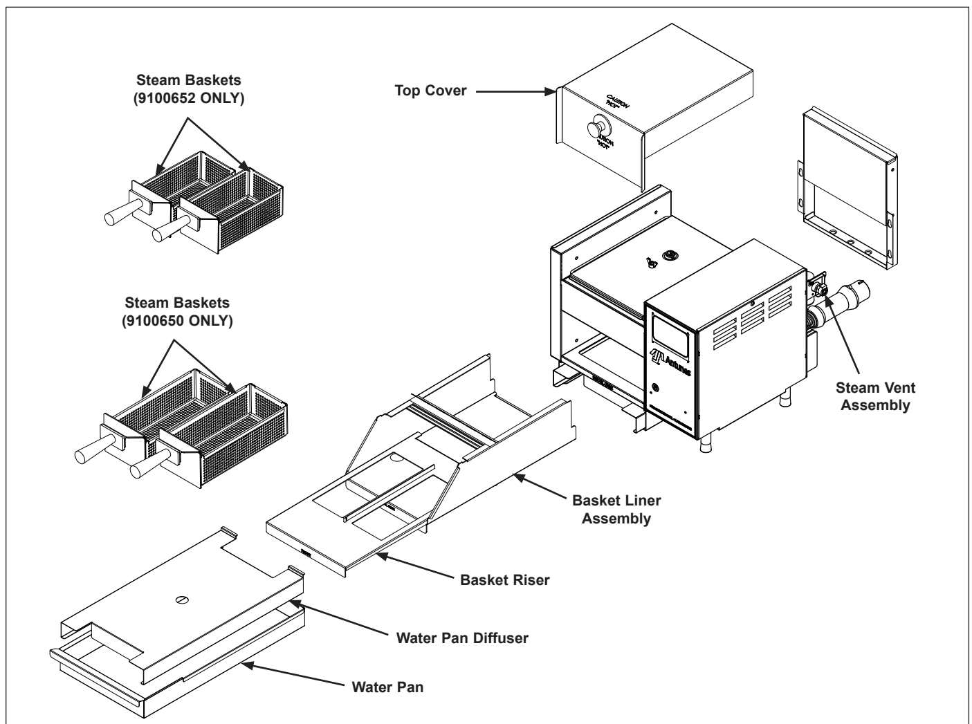
Figure 4. Components
