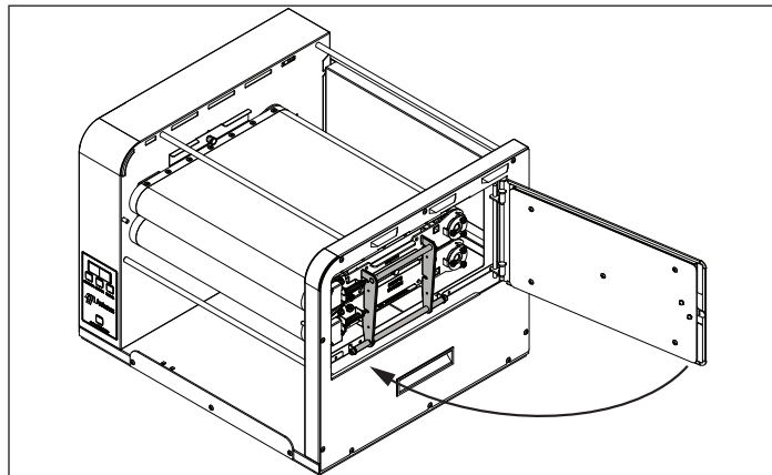
Figure 8. Close and Lock the Side Panel
