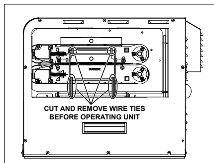
Figure 2. Remove Wire Ties
