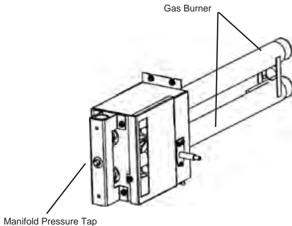
Figure 2-17. Burner Assembly
