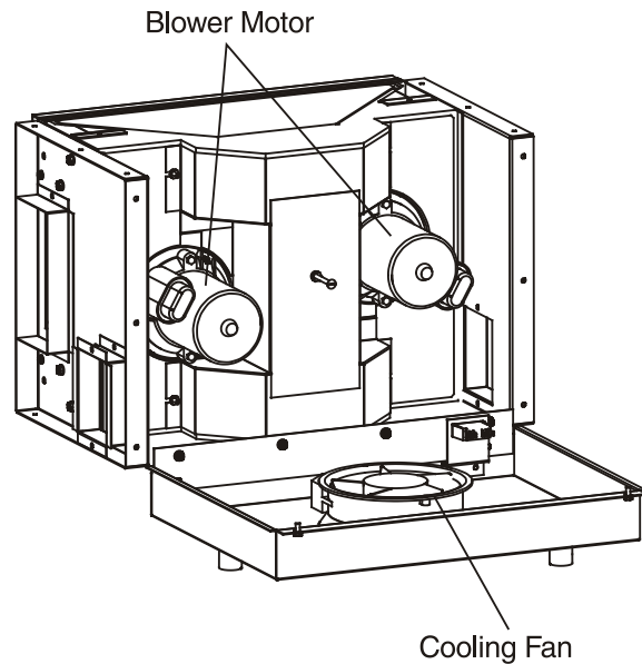
Blower Assembly
